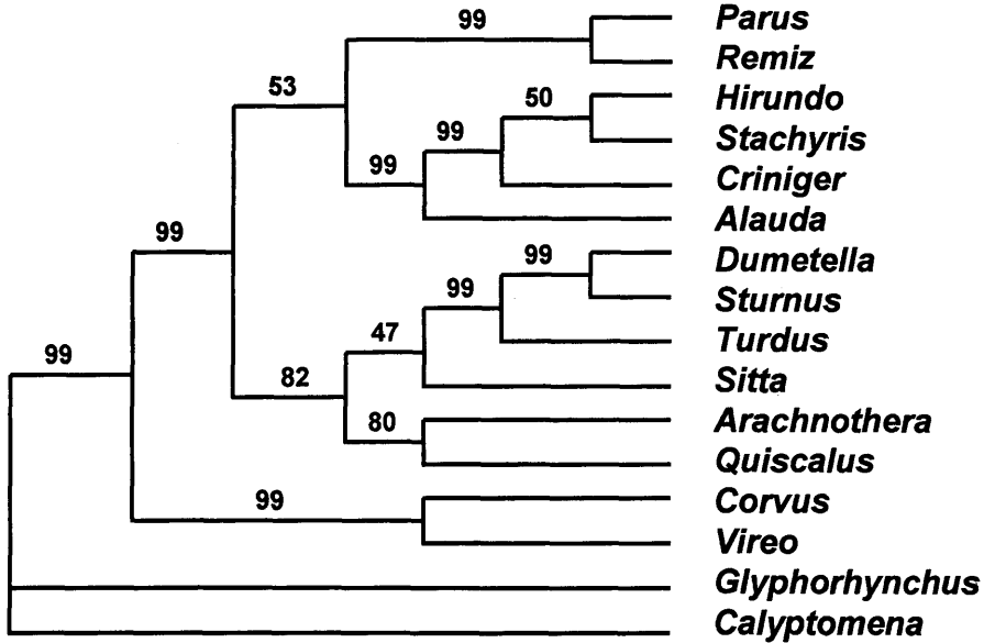
FIGURE 6. Bootstrap majority rule summary of the complete 16-taxon matrix of passerines produced from 1,000 pseudomatrices (Krajewski and Dickerman, 1990) using the PHYLIP (3.4) CONSENSE program (Felsenstein, 1989). Numbers are percentages of branch support.
