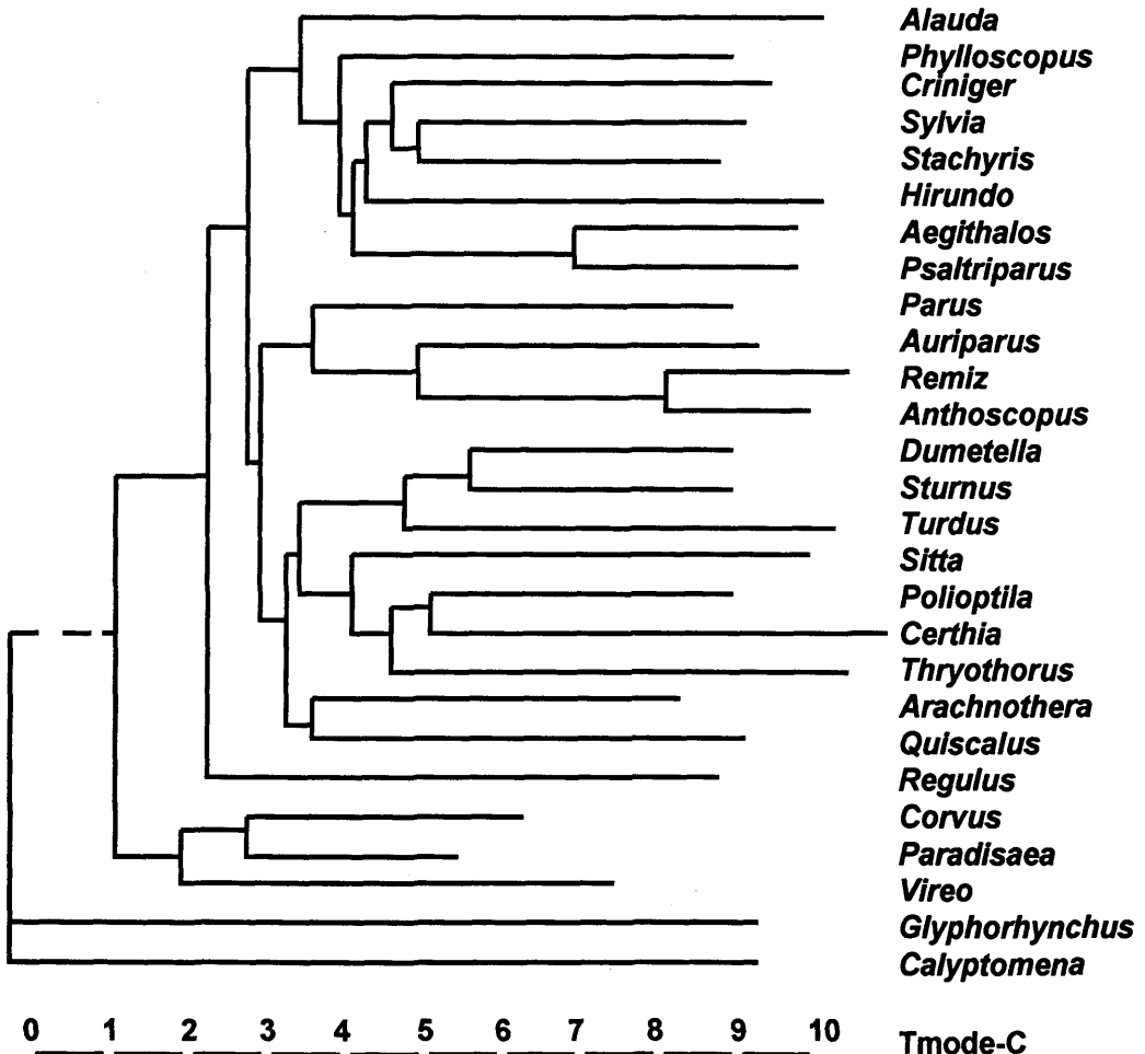
FIGURE 5. A summary weighted least squares (Fitch and Margoliash, 1967) DNA-hybridization tree for 27 passerines. This tree is primarily the best fit weighted least squares branching pattern from a 25-taxon \Delta T_{mode-C} folded matrix of DNA-hybridization distances. The position and branch length of Paradisaea were determined from a folded 17-taxon matrix consisting of Paradisaea and the 16 taxa in Figure 4. (Not enough Paradisaea DNA was available for comparisons with the remaining 10 species.) The branch lengths and the arrangement among Polioptila , Certhia , and Thryothorus were determined using the lacunose matrix method of Lapointe and Kirsch (1995, J. Kirsch, pers. comm.) because comparisons between Polioptila and Thryothorus failed for mechanical reasons.
